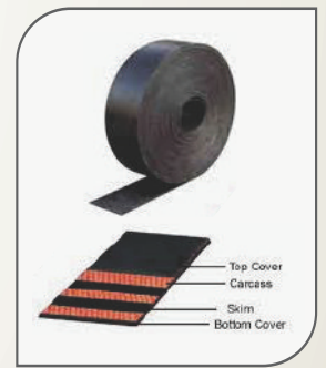
Elevator Belt per AS 4035
